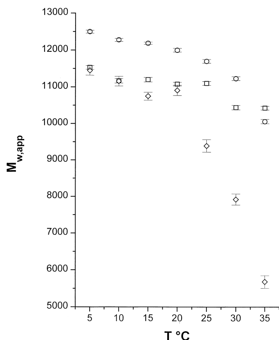
Fig. 2 The dependence of M_{w,app} on temperature at peptide concentrations of 310 ( \square ) 31 ( \circ ) and 3 \mu\text{M} ( \diamond ) in phosphate/fluoride buffer. An XL-A ultracentrifuge was used and the temperatures quoted are those reported by the instrument
